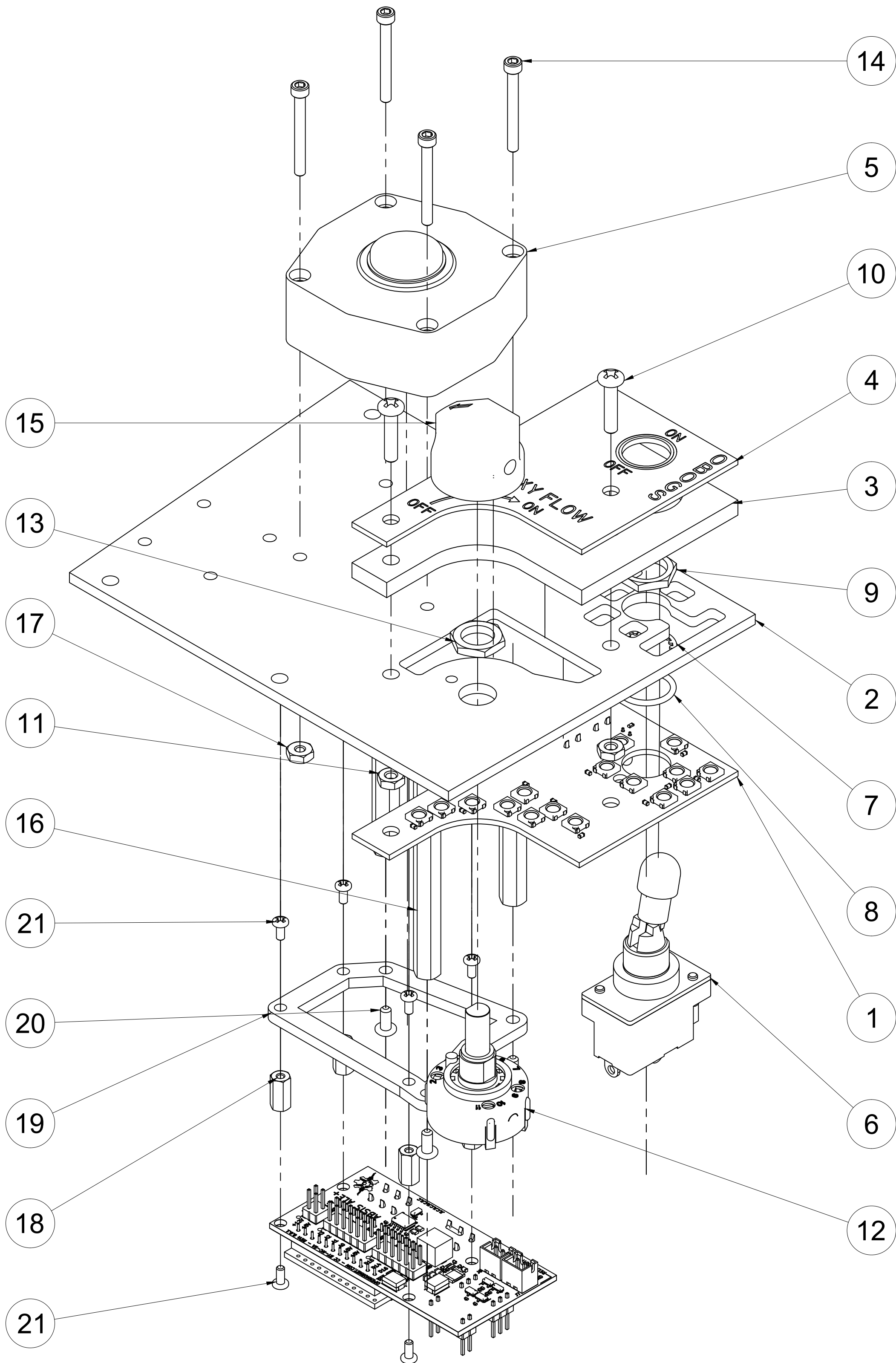
-1 ASSY SCALE 1.2:1
