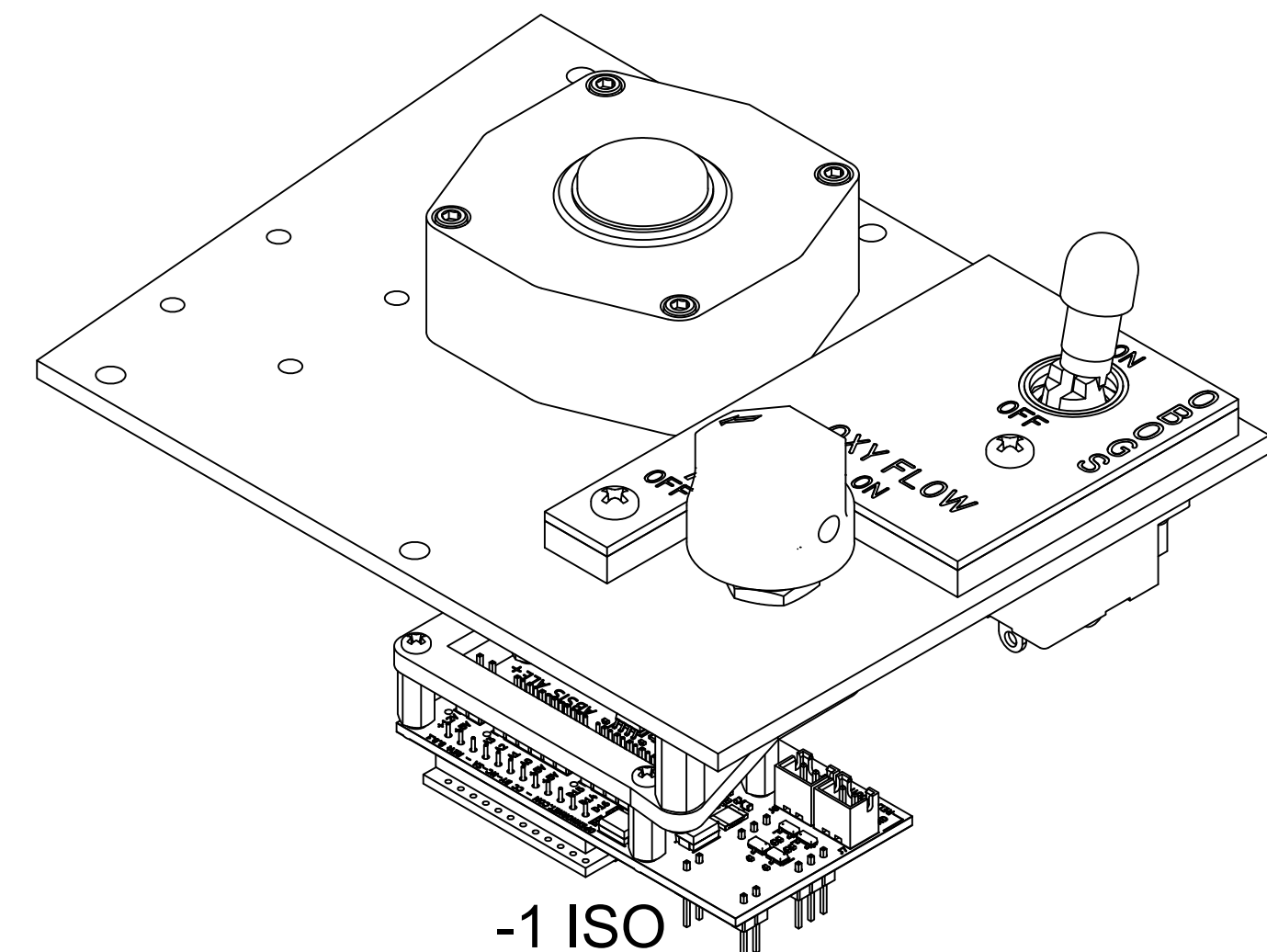
-1 ISO SCALE 1.2:1
